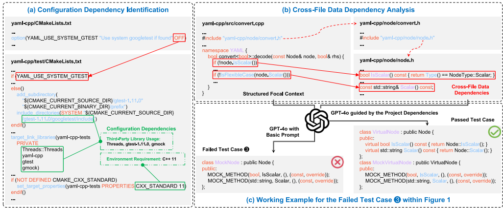
Fig. 4. Illustrative example of project-dependency extraction.
