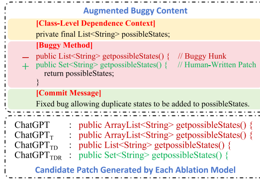
Fig. 11. An example from the augmented BFP benchmark only fixed by PATCH.
