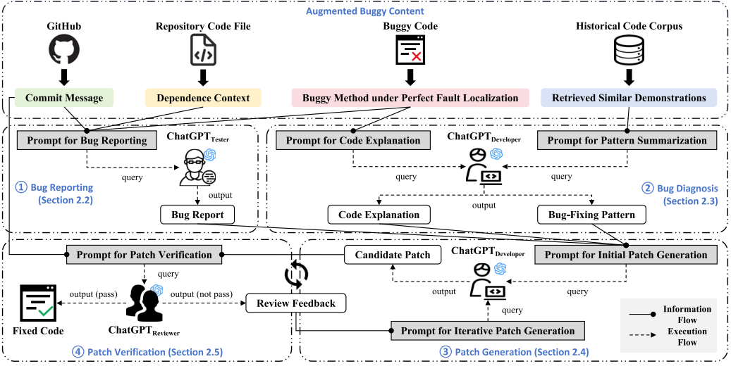
Fig. 3. Overview of PATCH.
