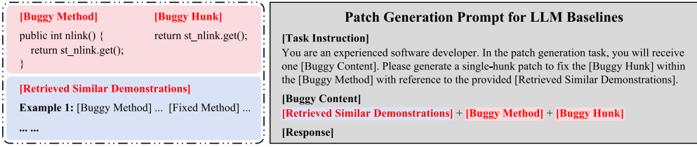
Fig. 9. A prompting example for the LLM baselines.
