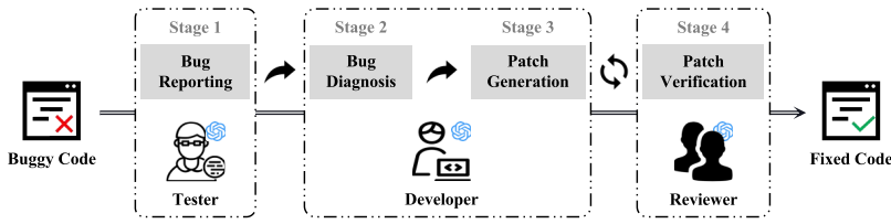
Fig. 2. The brief structure of PATCH.
