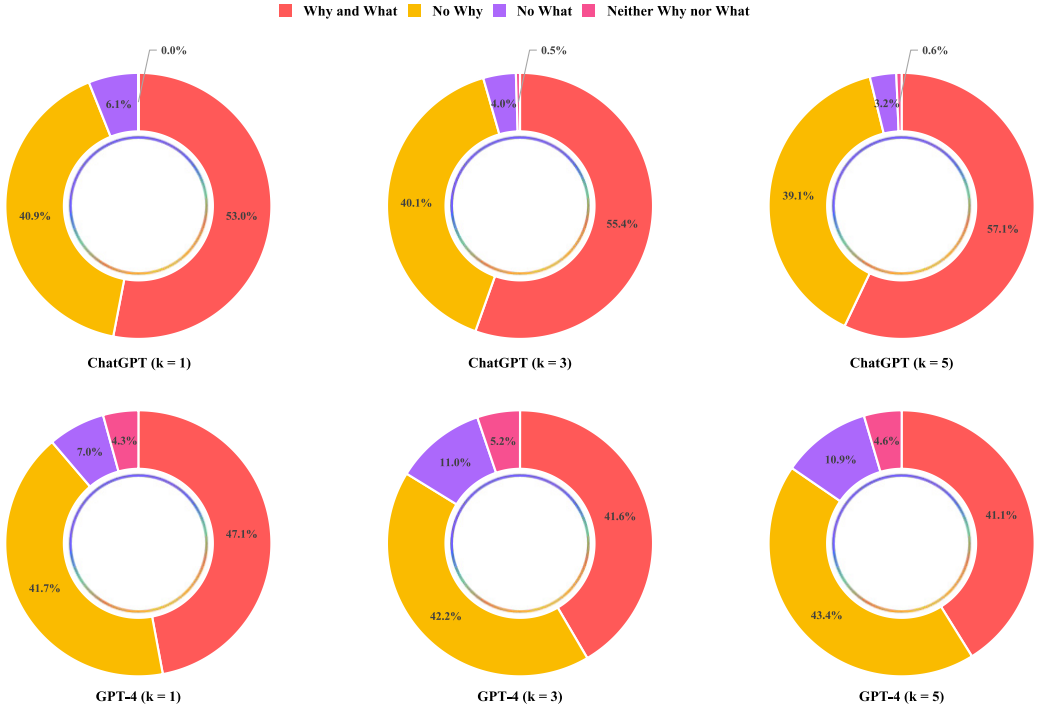
Fig. 12. The contribution of different CM types to improvements in bug-fixing performance.
