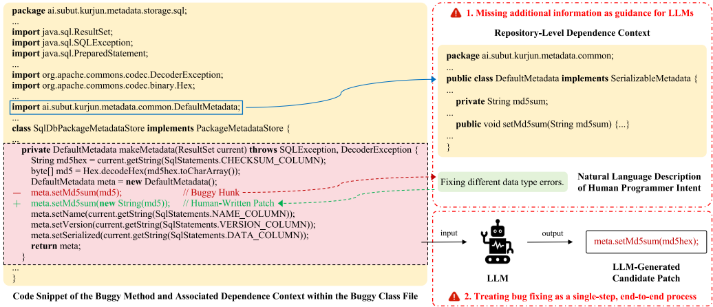
Fig. 1. Limitations of existing LLM-based bug-fixing approaches.
