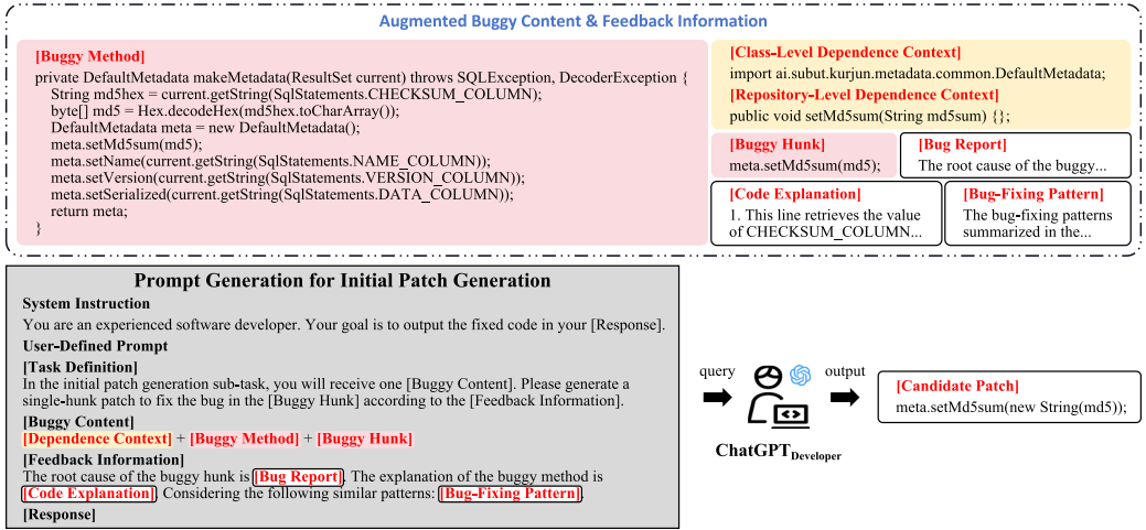
Fig. 7. A prompting example of the developer's behavior during the initial patch generation stage.
